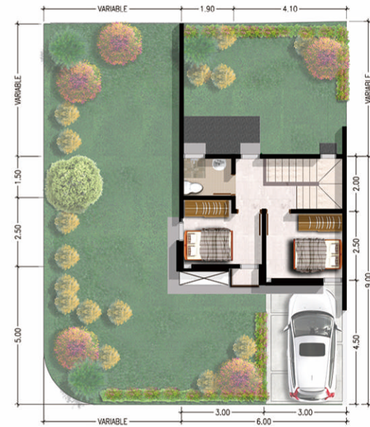
Denah Lantai 2
