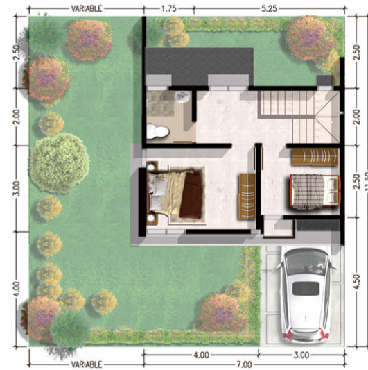
Denah Lantai 2
