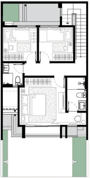
THIRD FLOOR
