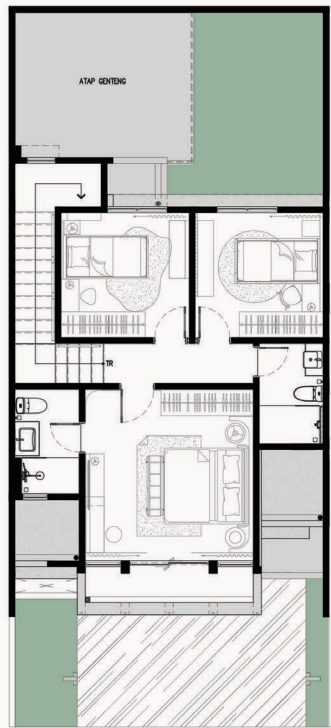
THIRD FLOOR
